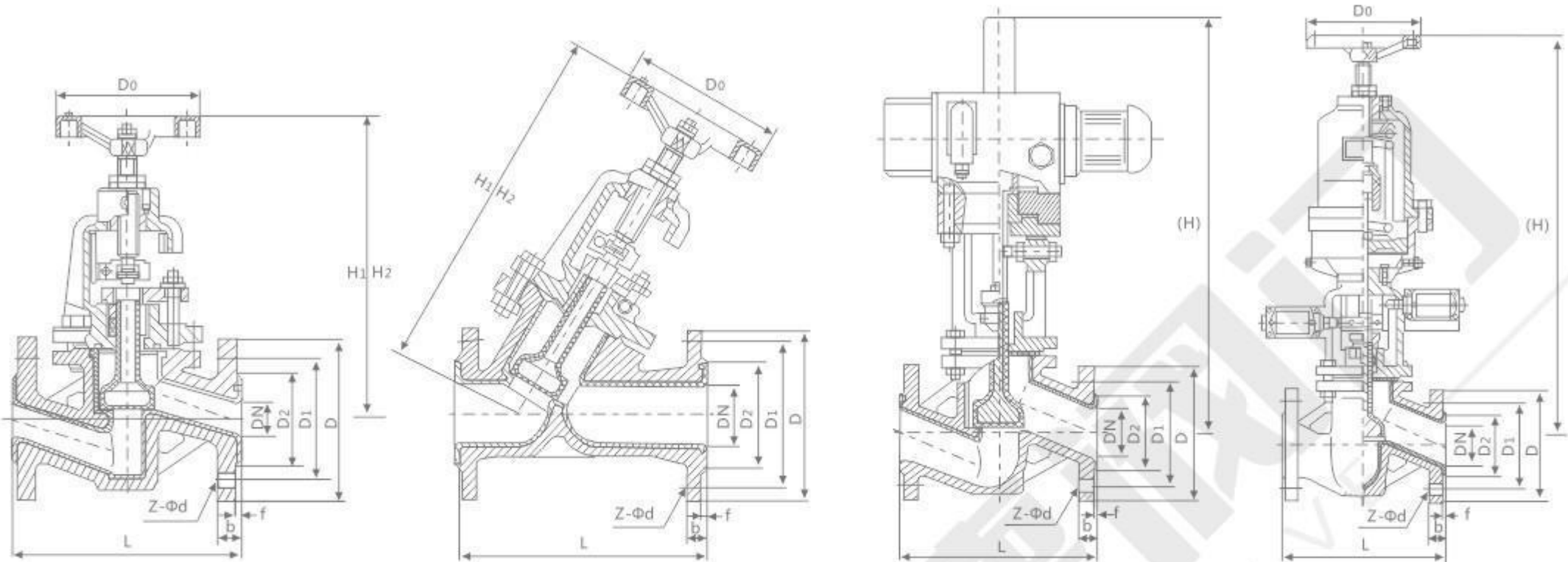
J41 F3 F46 型Type 法兰连接手动截止阀（直通式） Flange connection manual cut-off valve (straight-through) J45 F3 F46 型Type 法兰连接手动截止阀（直流式） Flange connection manual cut-off valve (DC type) J941 F3 F46 型Type 法兰连接电动截止阀（直通式） Flange connection electrically operated cut-off valve (straight-through) J6B41 F3 F46 型 法兰连接气动截止阀（常闭式） Flange connection air operated cut-off valve (Normally closed)
