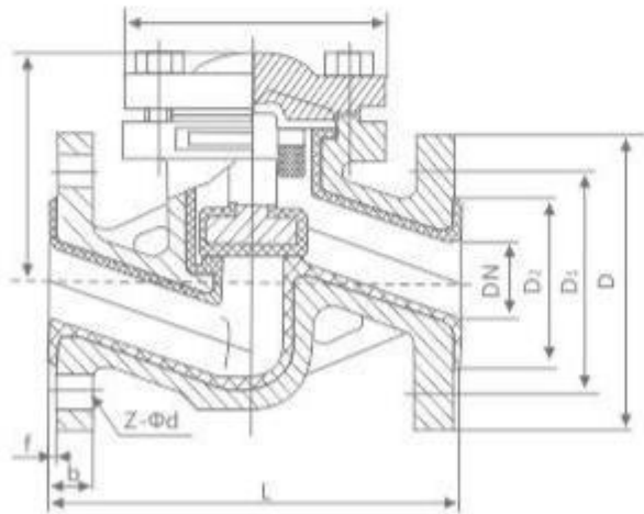
H41-F 46 型法兰连接止回阀(直通升降式) H41-F 46 Flange connection valve (straight-through lift)
